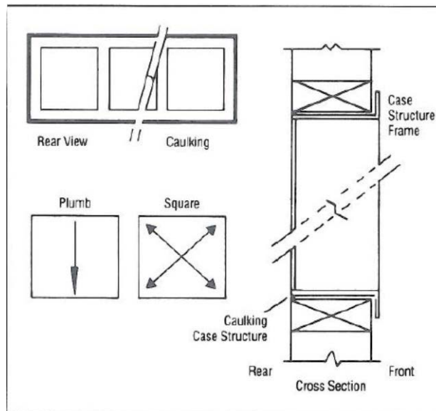
Frame Installation
