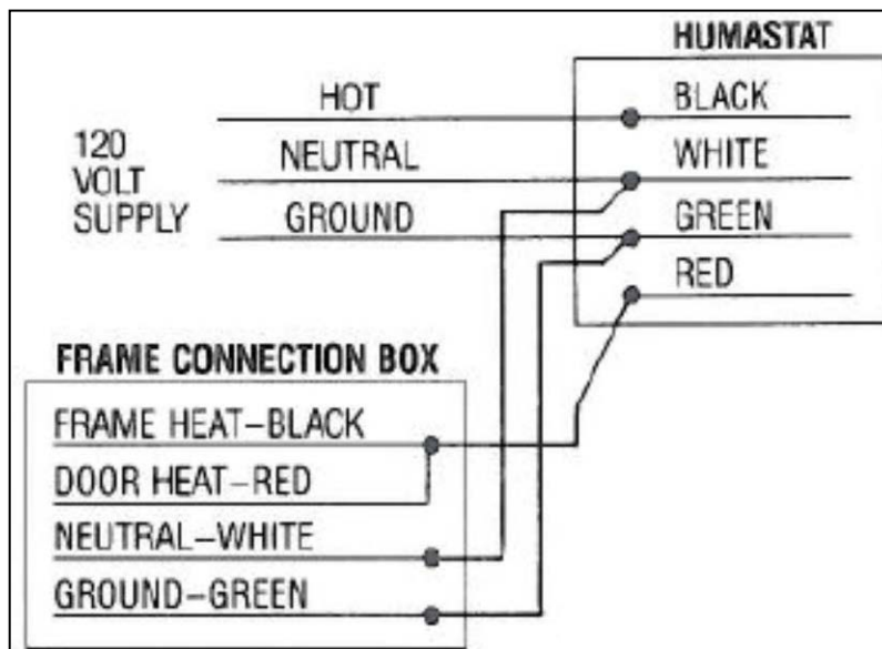
Wiring Diagram
